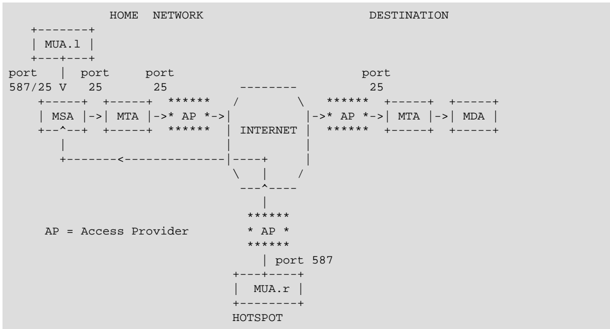
Figure 1: Example of Port 587 Usage via Internet
